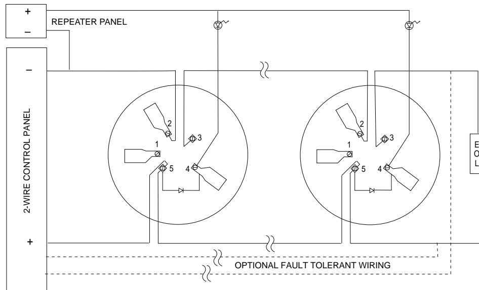
Figure 2. Typical wiring diagram for 2-wire detector systems:
