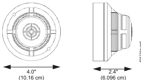
FSC-851 IntelliQuad Advanced Multi-Criteria Detector
