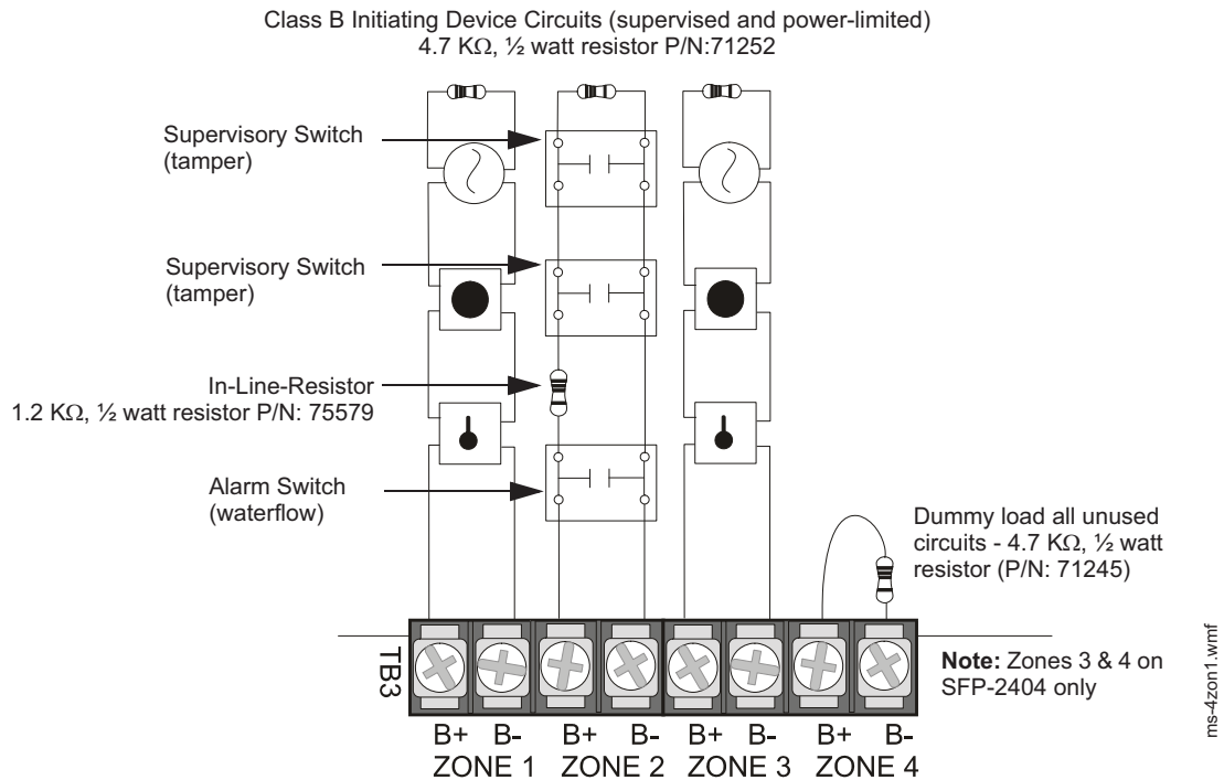
Figure 2.5 Style B Combination Circuit on Zone 2 of the SFP-2404
