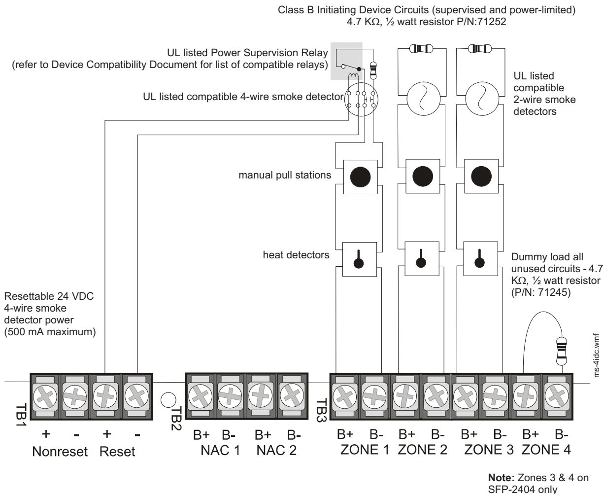
Figure 2.4 IDC Connections
