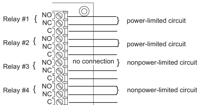
Figure 2.14 4XZM Zone Relay Module
